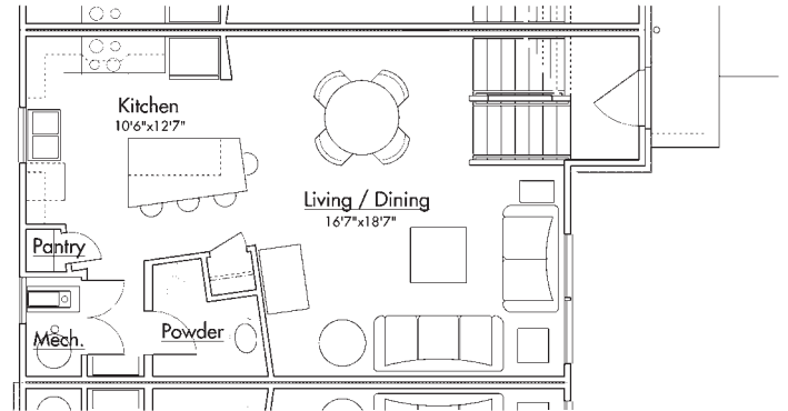
First Floor Gross Area: 603 s.f.
