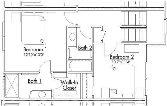
Second Floor Gross Area: 601 s.f.
